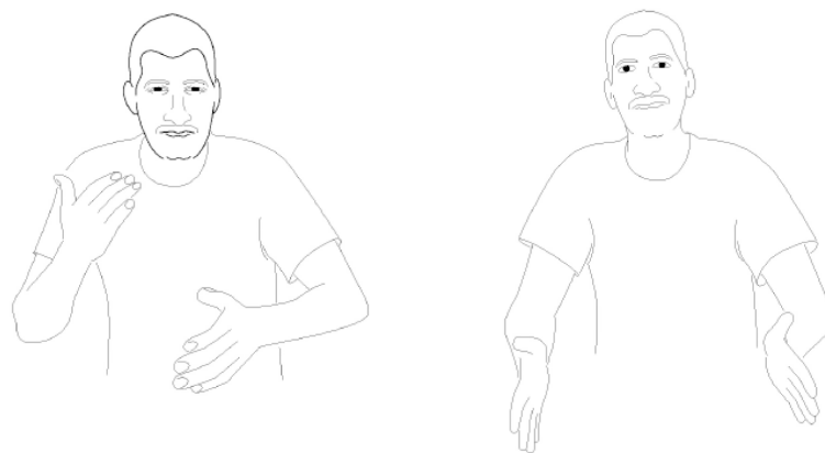
Figure 4. ABSL (a) BUILD and (b) WALLS, separated by prosodic break
