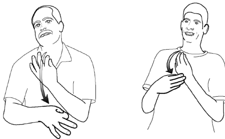
Figure 2. ABSL BANANA (a) with B handshape and (b) with N handshape
