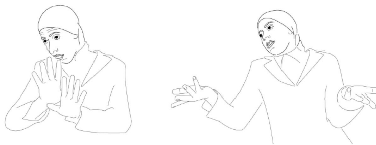
Figure 5. ASL characteristic conditional prosody. (a) (If) NO, (b) (then) NOTHING-TO-DO (“If he says, ‘No,’ then there’s I can do about it.”)
